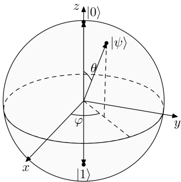
Figure 1: Bloch sphere
