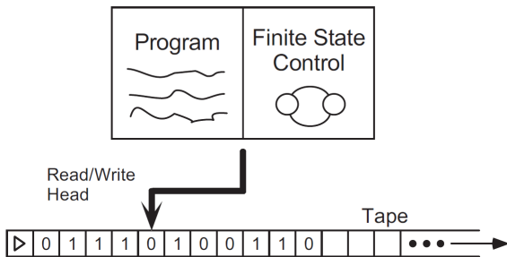
Figure 6: A Turing machine.
