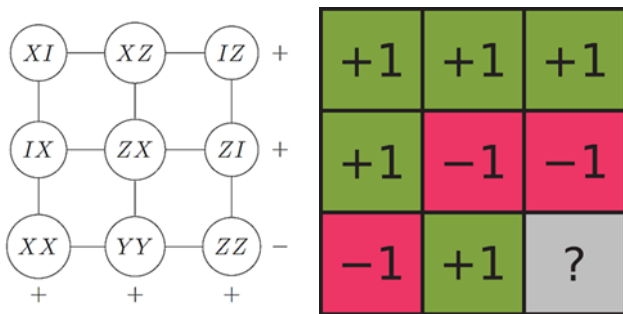
Figure 5: Mermin-Peres square.
