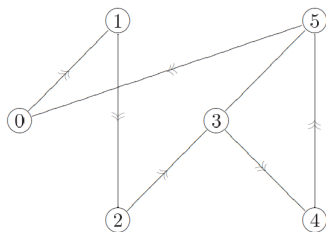
Figure 9: A Hamiltonian cycle
