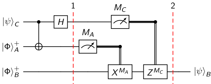
Figure 4: Quantum teleportation
