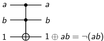
Figure 11: NAND gate.
